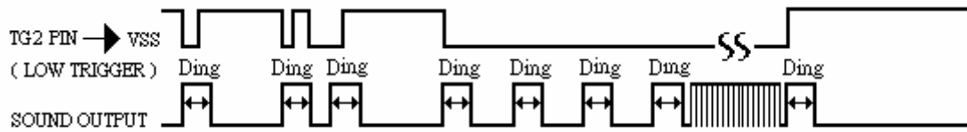
TRIGGER MODE : ONE SHOT RE-TRIGGER
