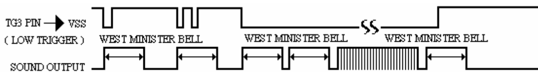
TRIGGER MODE : ONE SHOT RE-TRIGGER
